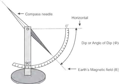
Fig. 12.7: Magnetic inclination.
